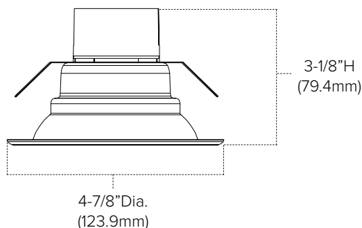
E4 Module Profile View
